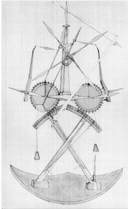
COMBINED THERMOMETER, HYGROMETER, BAROMETER AND PYROMETER Invented by the author in his boyhood
